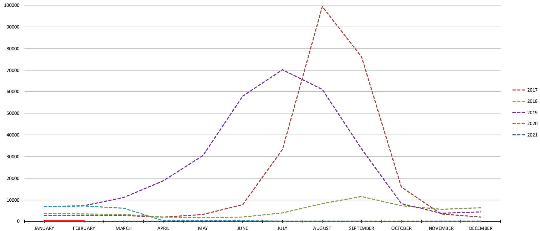
ANNUAL AUSTRALIAN LABORATORY CONFIRMED FLU NUMBERS
